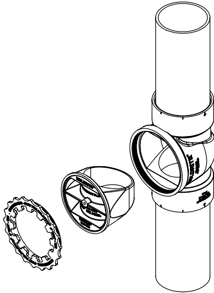
Cleanout Mode with Cleanout Plug
