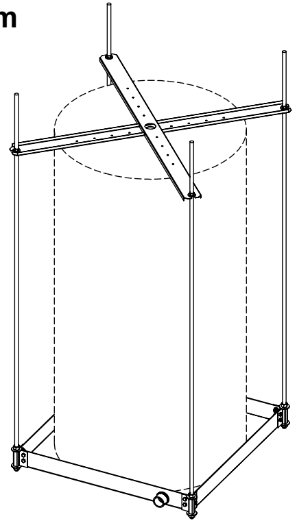
FULLY ASSEMBLED
