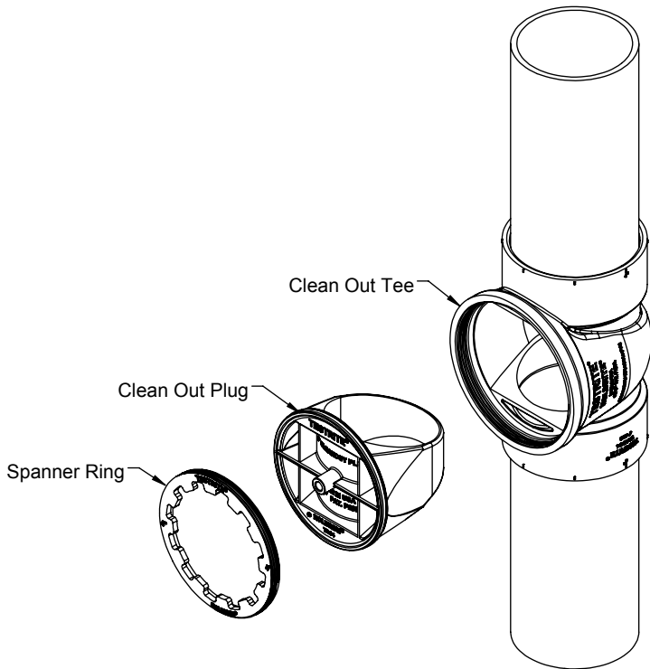
Cleanout Mode with cleanout plug
