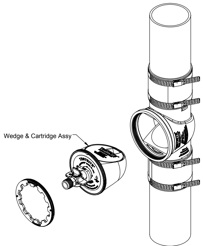
DWV Test Mode with TestRite® Wedge
