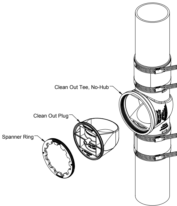
Cleanout Mode with cleanout plug
